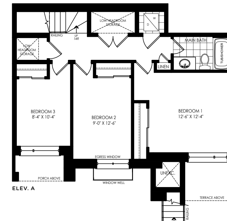
OPT. 3 BEDROOM GROUND LEVEL
