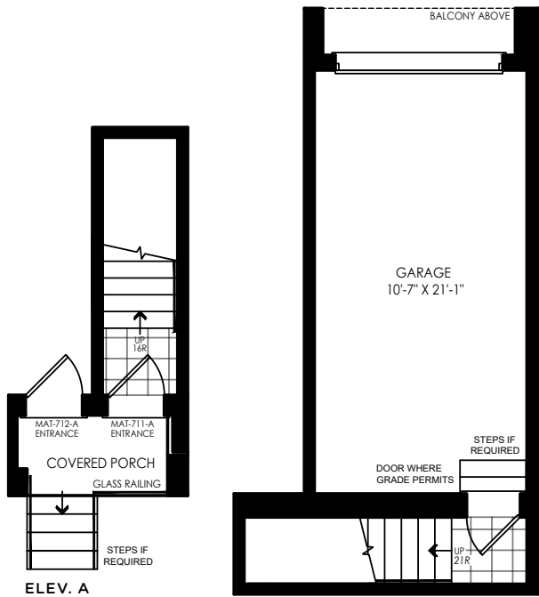
FIRST LEVEL (Front) GARAGE LEVEL (Rear)
