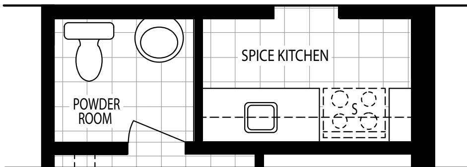
PART. GROUND FLOOR PLAN WITH OPT'L. SPICE KITCHEN, ELEVATION C
